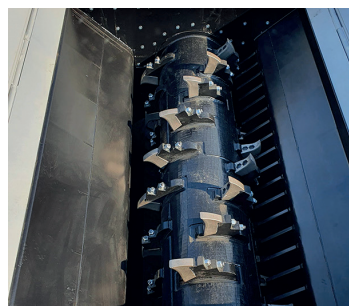
Shredding Unit
